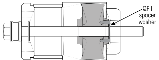
Figure 3: QF I spacer washer (as shown in Hendrickson literature number L427)
