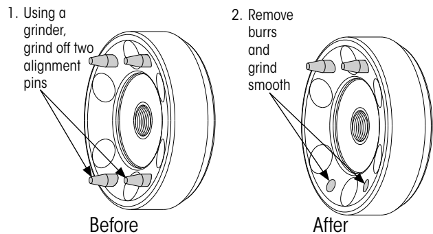
Figure 2: Rear drive plate modification
