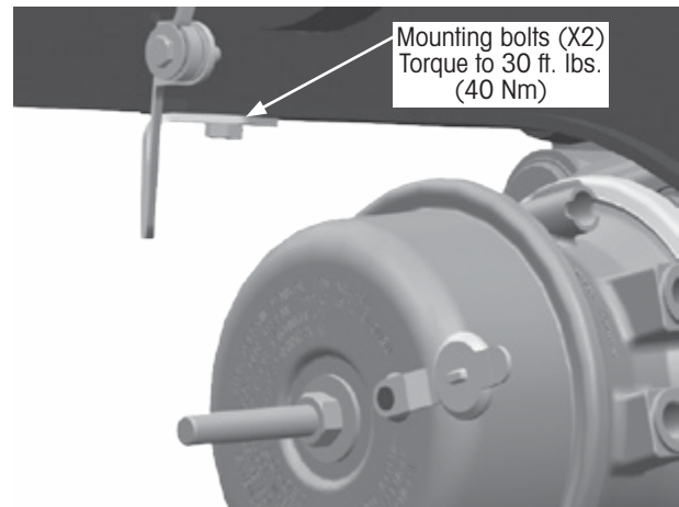
HCV lower linkage assembly with new bracket
