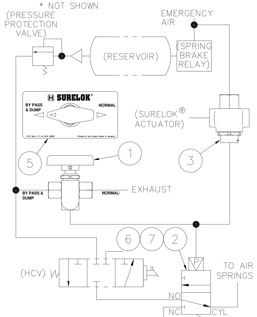
AK-198 - BYPASS VALVE & DUMP
