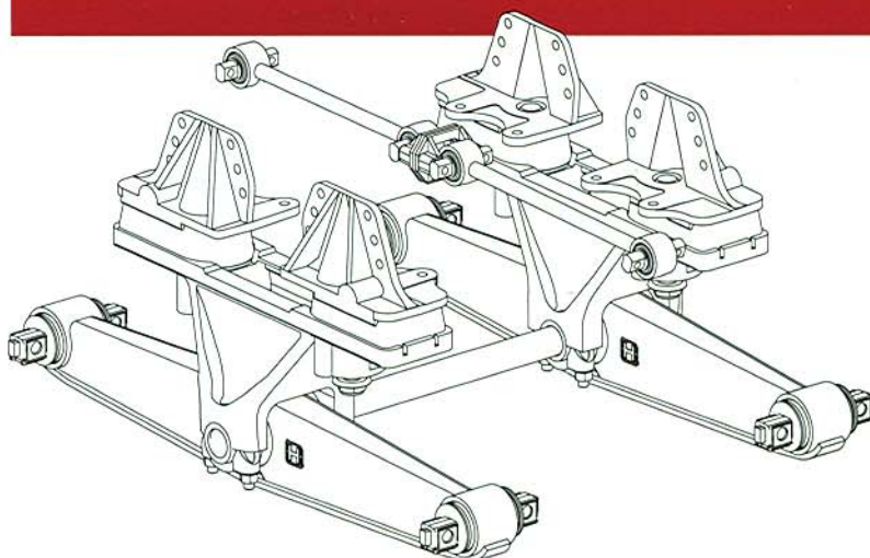
SUSPENSION SPECIFICATIONS
