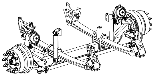
SOFTEK® with STEERTEK Axle equipped with Drum Brakes
