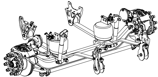
AIRTEK® with STEERTEK™ NXT Axle equipped with Air Disc Brakes
