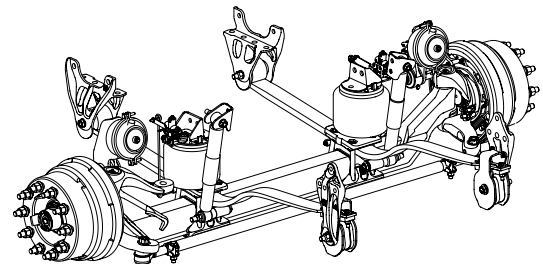
AIRTEK with STEERTEK Axle equipped with Drum Brakes
