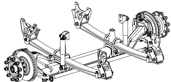
SOFTEK with STEERTEK Axle equipped with Air Disc Brakes
