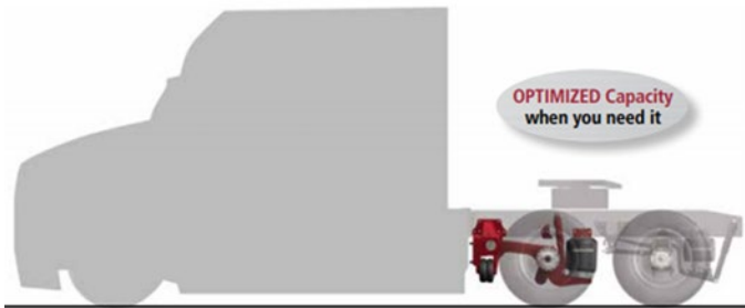
Axle lowered for 6x2 configuration – OPTIMAAX senses heavier load and lowers the non-driven axle
