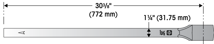
Spacer End Part No. 64474-000
