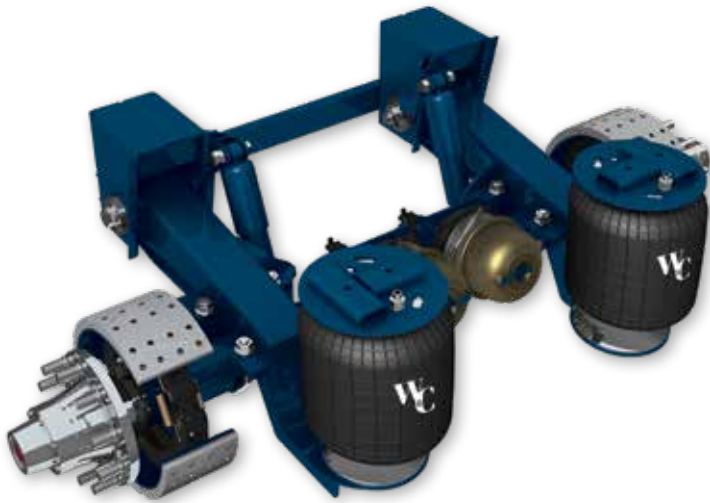
Low Mount
