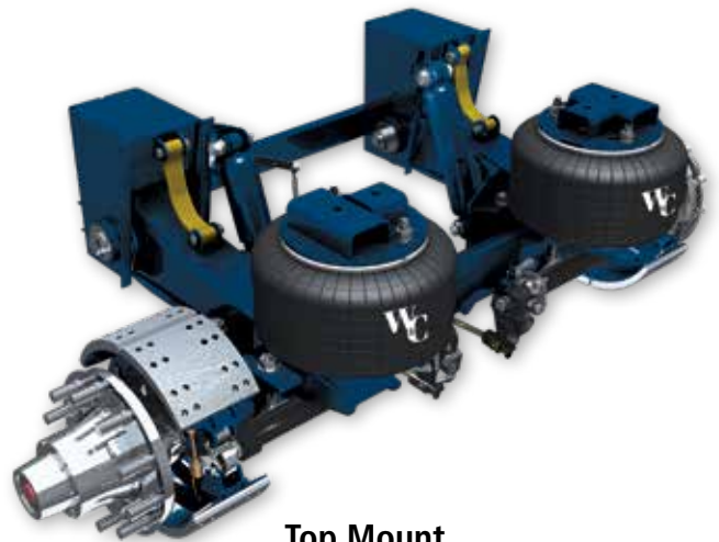
Top Mount
