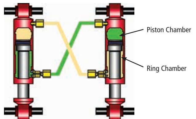
Cross Plumbing between Spring Cylinders
